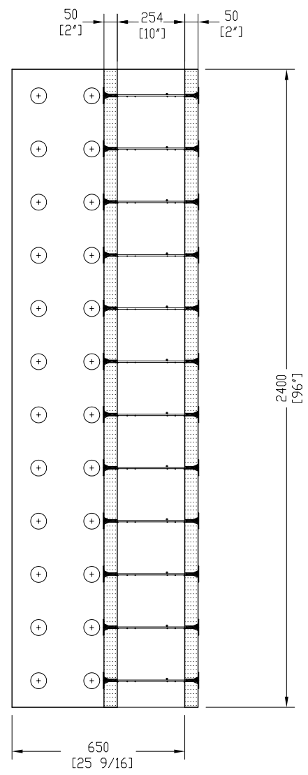
SIDE VIEW
