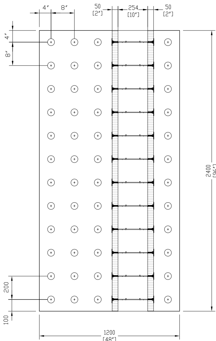
FRONT VIEW
