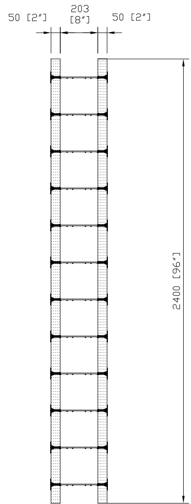
SIDE VIEW
