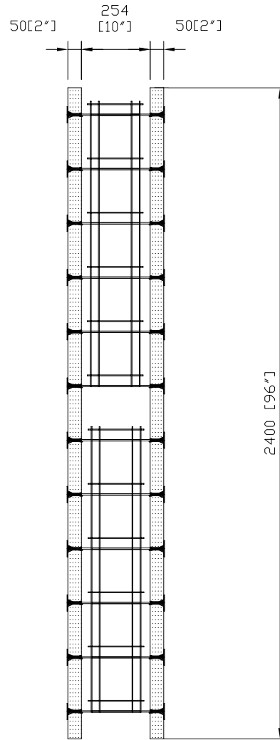
SIDE VIEW
